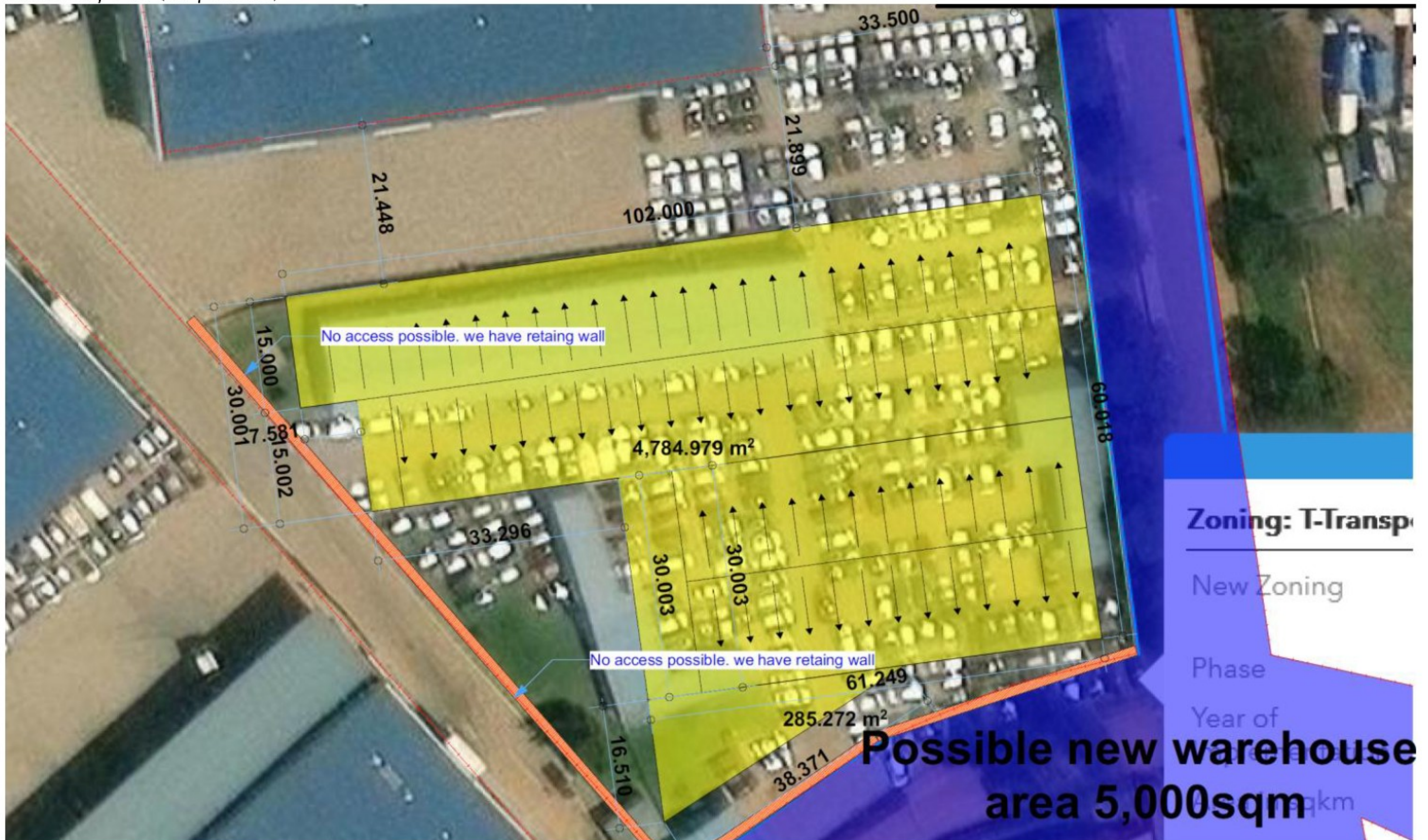
Site Layout (in yellow)
